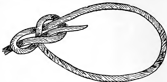
FIG. 58.—Bow-line.
